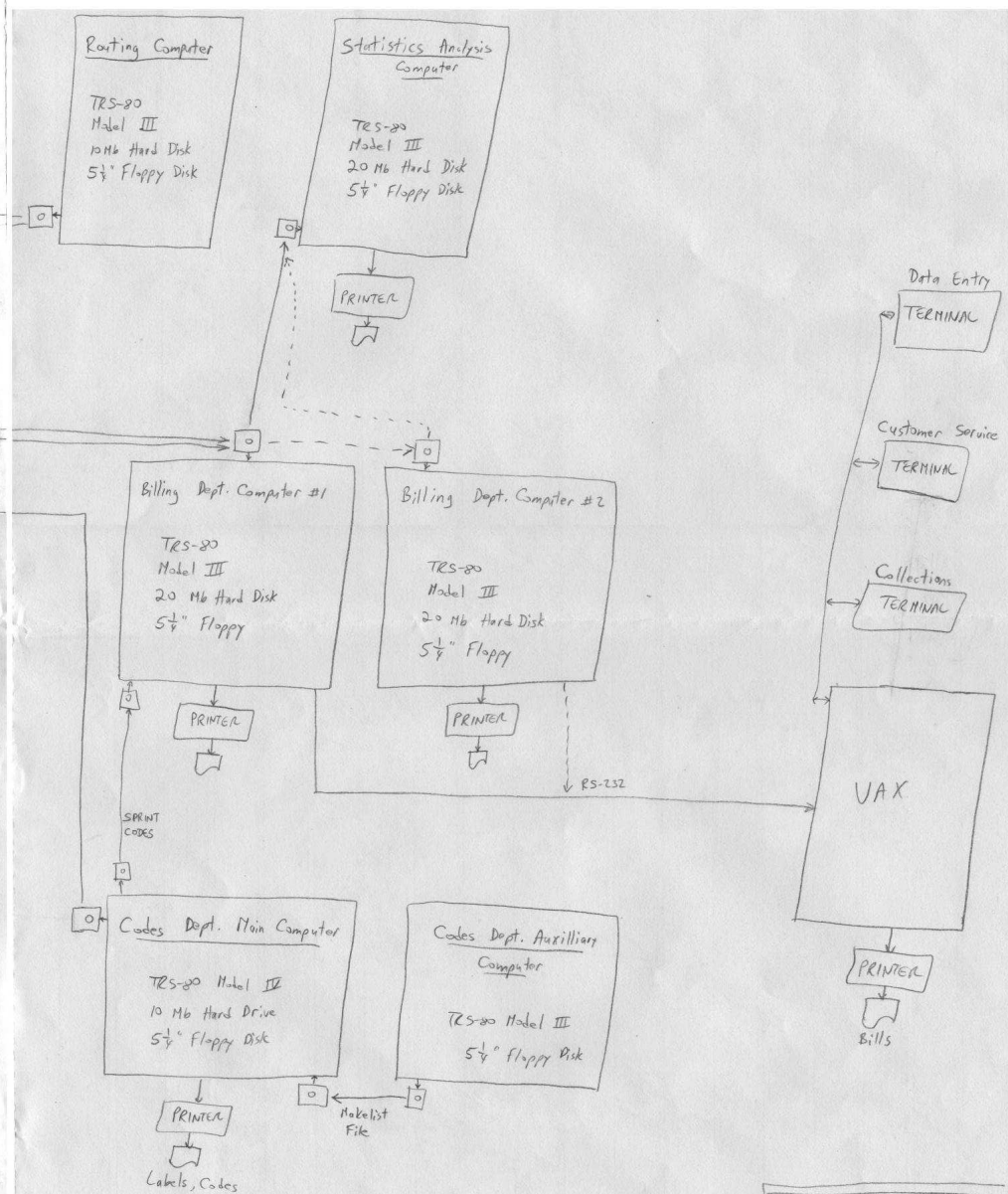
Current Telecomm Switch and Computing Facilities 2-7-84
